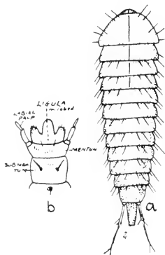
Fig. 194. a, Scaphisoma convexum Say; b, Ventral aspect of labium.
